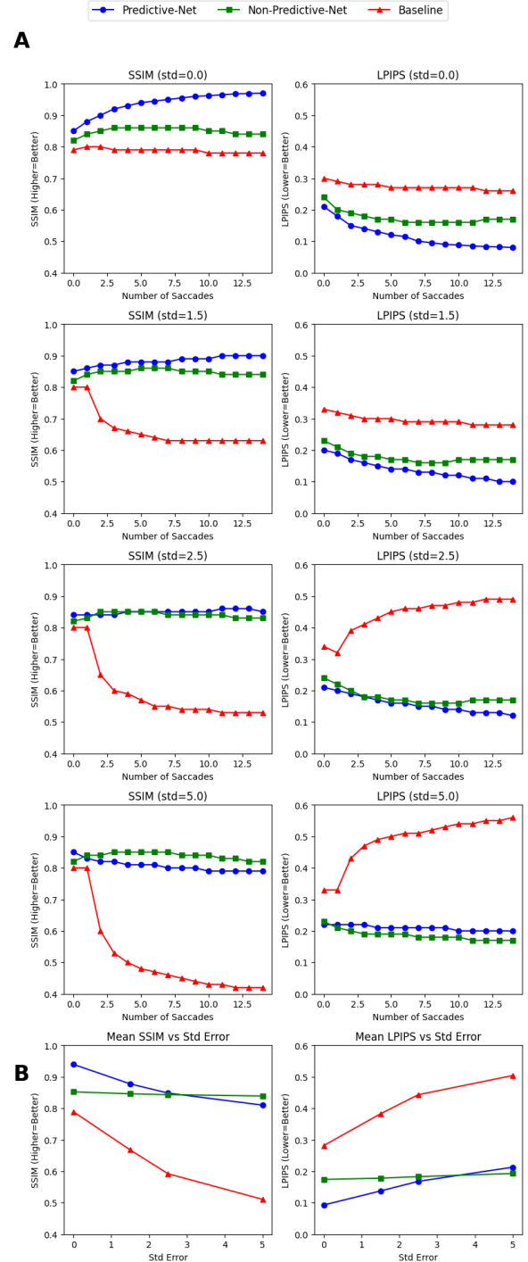
Figure 4: Performance evaluation of predictive and non-predictive Models under varying Saccades and error variability.
