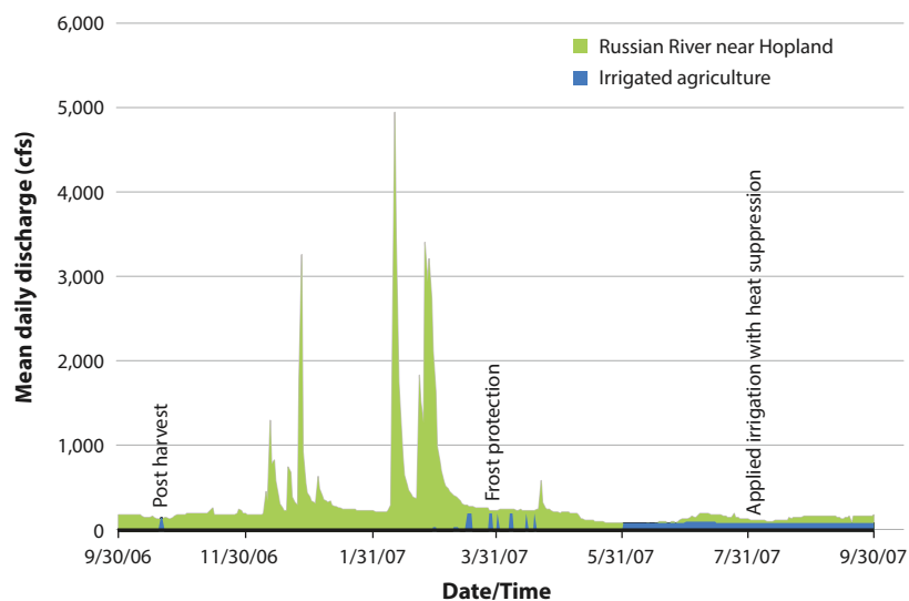
FIG. 7. Mean daily discharge (green) from Oct. 1, 2006, to Sept. 30, 2007, at USGS stream gauging station #11462500 near Hopland, California, and estimated daily rates of water applied (blue) to meet irrigated agriculture's water demand in the Mendocino County portion of the Russian River watershed.
