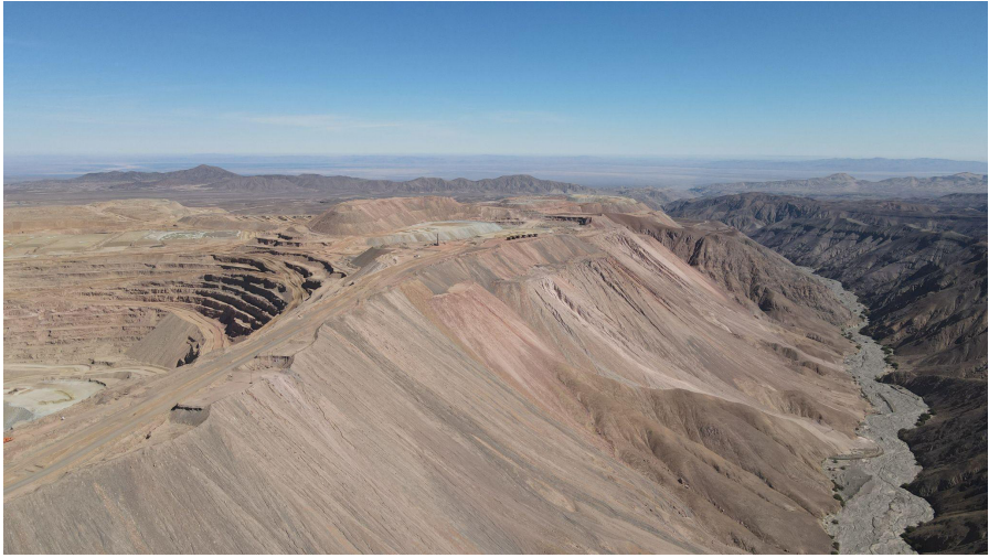
FIGURE 2. Impact of mining on the Quipisca watershed. Photo by Juan Andrés Moraga Nova.
