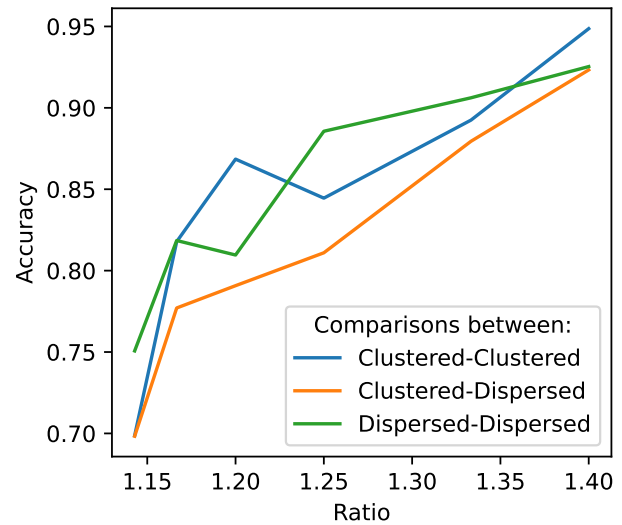
Figure 2: Participants' accuracy on the magnitude comparison task as a function of the ratio between the sets of points. Participants were less accurate on comparisons with stimuli of different cluster structures (Clustered vs Dispersed) than those with the same cluster structure (Clustered-Clustered & Dispersed-Dispersed).
