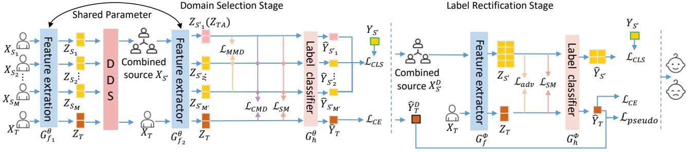
Figure 1: The architecture of DDSPR model. The entire model is primarily divided into two main modules: (1) Domain selection stage : Generate the combined source domains and the determined pseudo-labels for the target domain. (2) Label rectification stage : Correct incorrect target domain pseudo labels and evaluate the prediction results.
