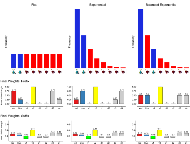
Figure 1. Distribution of fribbles which occur with affix "ma" in each of the three input sets: flat (as in Vujovic et al., 2021) exponential and balanced exponential. The distribution will be mirrored for the alternative affix (“ge”), with output
