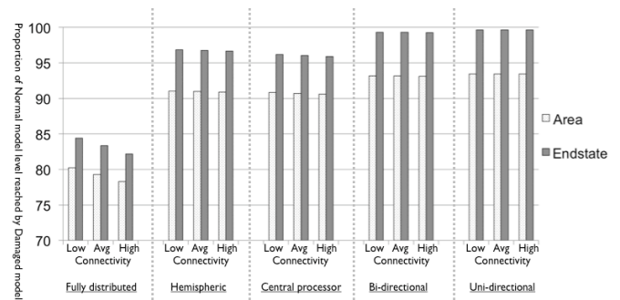
Figure 3: Proportion of Area and Endstate obtained in peripherally-damaged models by level of Connectivity.
