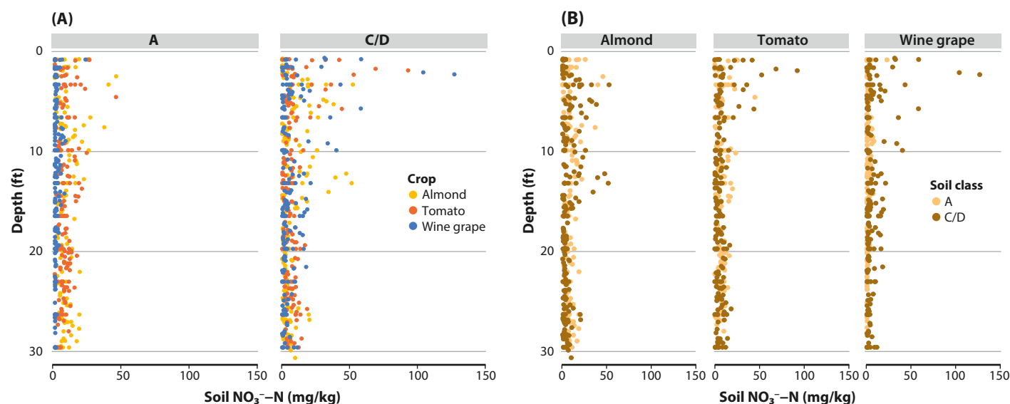
FIG. 2. Soil \text{NO}_3^- -N profiles (ug \text{NO}_3^- -N/g soil) down to 30 feet by (A) crop and (B) soil class ( n = 1,058 ).
