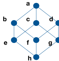
Figure 3: Geometric configuration of a Hasse diagram.
