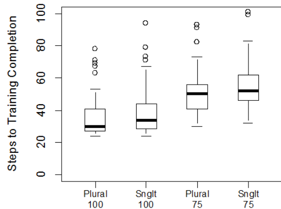
Figure 2: Boxplots of number of steps to completion of the training phase for each condition. The 100 conditions are represented on the left, 75 conditions on the right.
