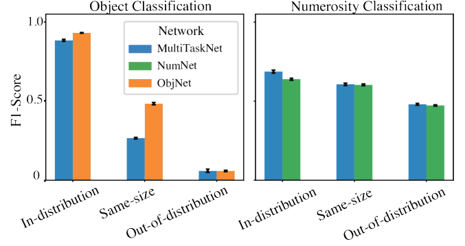
Figure 2: Overall performance (Macro F-1 Score) on classification of object and numerosity, for each type of network.
