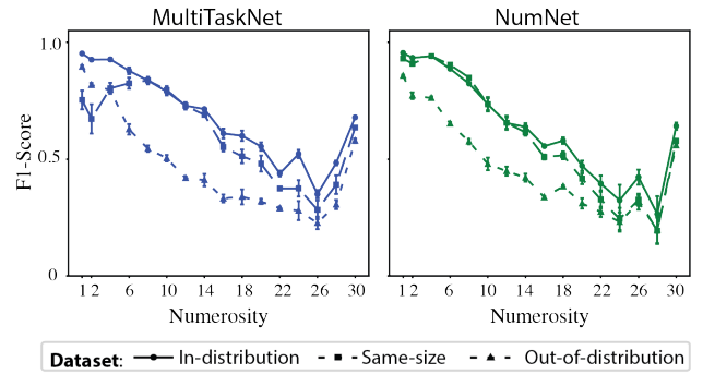
Figure 3: Performance on each numerosity class.
