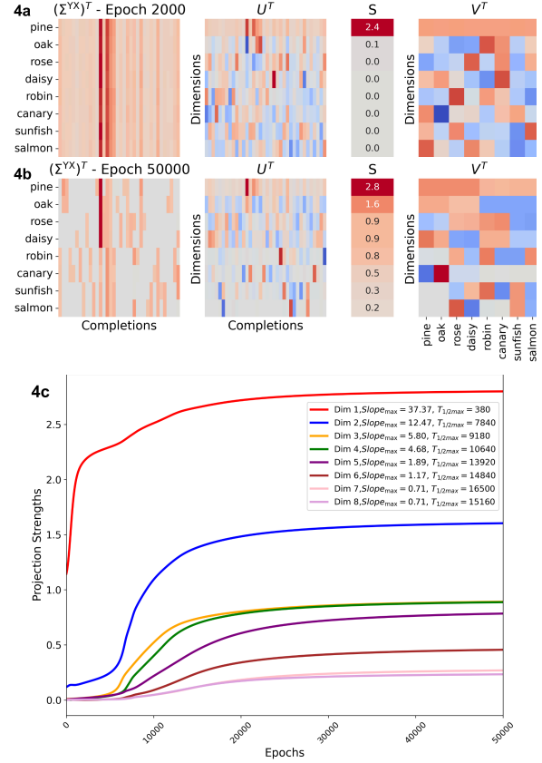
Figure 4: Transformer Activations Decomposition. (a,b) SVD on activations at epochs 2k and 50k. (c) Strengths of projections of \Sigma^{YX} onto dimensions of \Sigma^{\text{OI-CP}} for dimension curve with the median max slope, across seeds. Max slope (multiplied by \tau ) and time of half max (in epochs) in legend.
