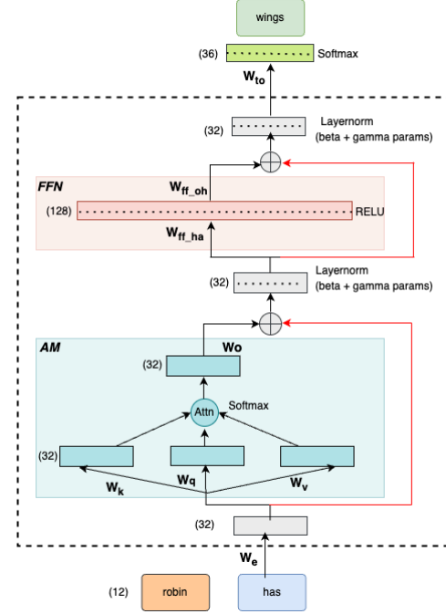
Figure 2: Minimal Transformer. Numbers show layer size. Modifiable parameters include weight matrices (e.g. W_e ) and LayerNorm unit-wise \beta and \gamma parameters.
