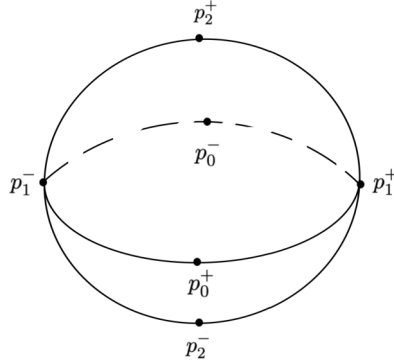
Figure 1: Two sphere in \mathbb{R}^3 with six critical points of the Morse function f = x^2 + 2y^2 + 3z^2 .
