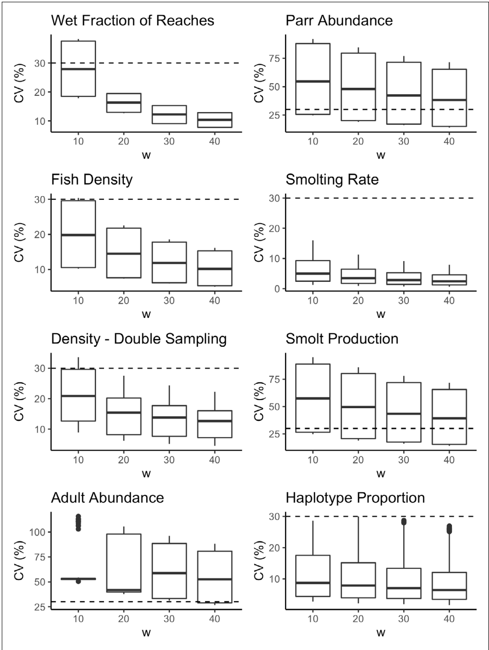
FIGURE B-1. Uncertainty (coefficient of variation) for selected estimators from the test simulations, as a function of number of reaches sampled ( w ). Dashed line marks the target CV of 30%.
