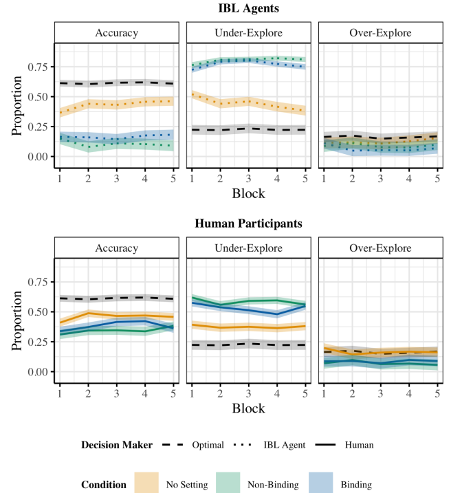
Figure 2: Accuracy, under-exploration errors, and over-exploration errors for optimal agents and IBL agents (top), as well as human participants (bottom), over blocks of 10 problems by condition. Error bars represent standard errors.
