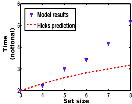
Figure 3: While our model differs from existing process models in predicting increasing response time as a function of choice set size, it does not converge to Hick's law's prediction of sub-linear increases.
