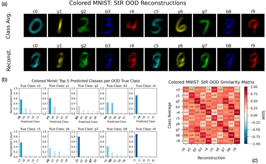
Figure 3: Modeling results for Experiment 2 (colored MNIST). (a) Signific-to-referential (StR) reconstructions of OOD referential input classes provided signific input only; class averages for each color-digit class. In-distribution (ID) composition reconstructions and class averages are not shown. (b) Top 5 referential-to-signific (RtS) predicted classes for each OOD true class. (c) SSIM values between StR reconstructions of OOD digit-color compositions and digit-color class averages.
